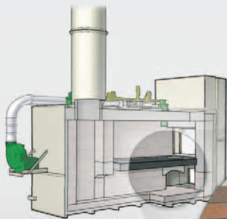
Quick Change Modular Hearth System
