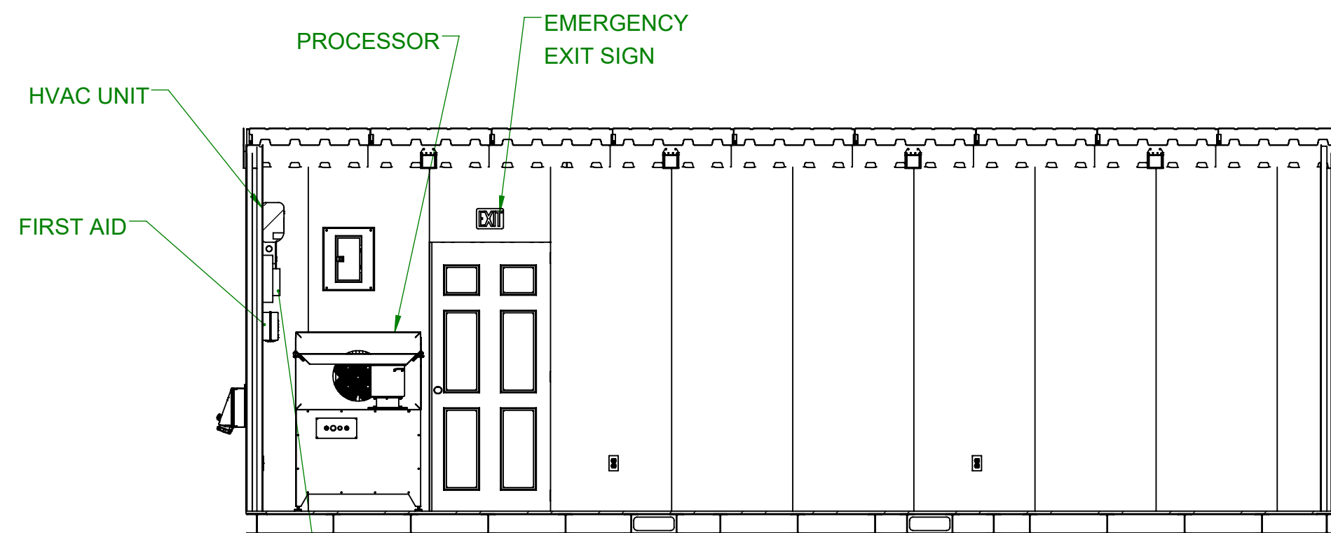
SECTION C-C
