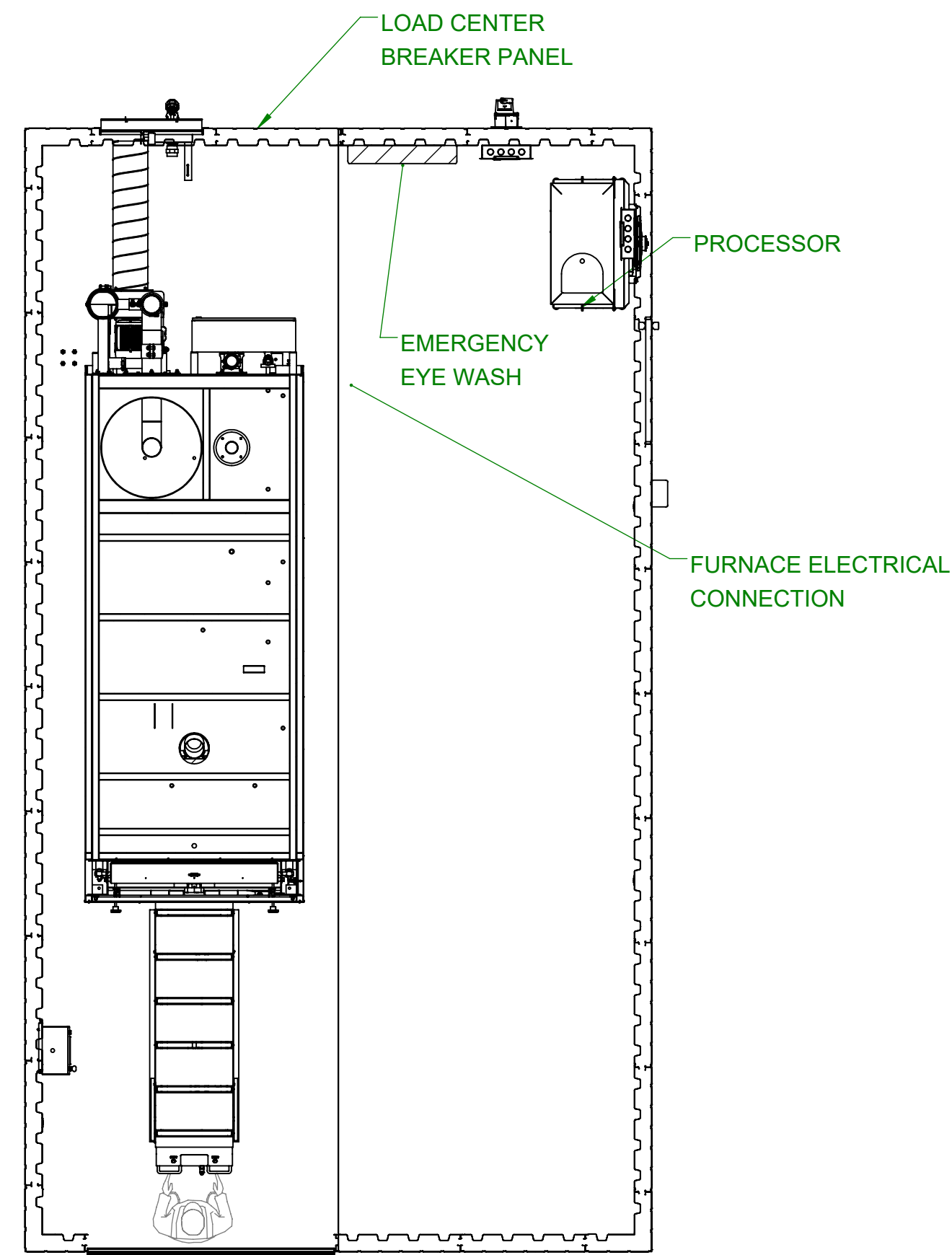
SECTION B-B
